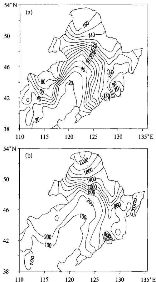
图 3 东北地区积雪日数(a,单位:d)和累积积雪深度(b,单位:cm)的分布 Fig. 3 Distributions of snow cover days (a,unit:d) and the cumulative snow depth (b, unit:cm) in Northeast China
