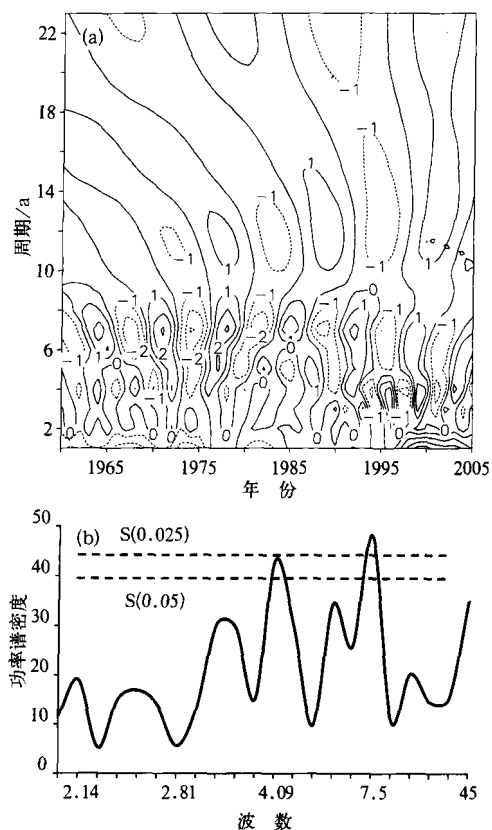
图 8 东北地区累积积雪深度时间序列的 Morlet 小波系数实部(a)和功率谱密度值(b) Fig. 8 Morlet wavelet coefficient (a) and power spectral density (b) of the time series of cumulative snow depth in Northeast China
