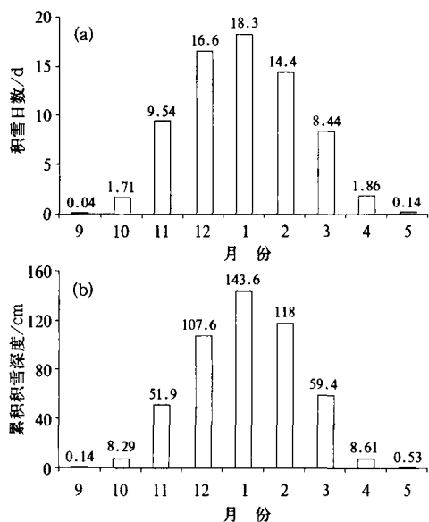
图 2 积雪日数(a)和累积积雪深度(b)的年变化 Fig. 2 Annual variations of snow cover days (a) and the cumulative snow depth (b)
